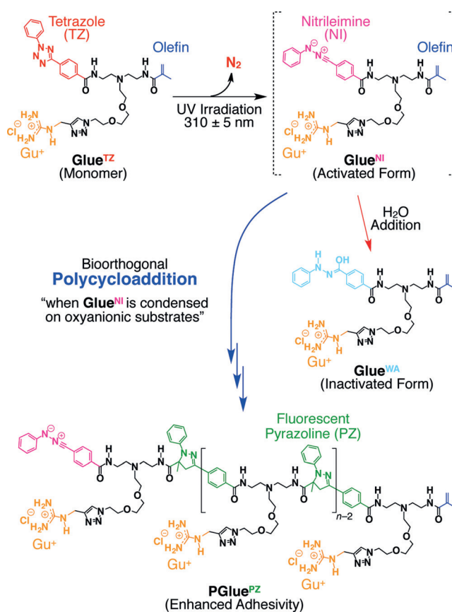
Scheme 1. A guanidinium ion (Gu + )-appended water-soluble monomer (Glue TZ ) carrying tetrazole (TZ) and olefinic termini, and its photochemical transformation into a nitrileimine-based reactive intermediate (Glue NI ) with elimination of N 2 , followed by bioorthogonal 1,3-dipolar polycycloaddition, thus affording a pyrazoline (PZ)-based fluorescent polymer (PGlue PZ ) carrying multiple Gu + pendants for enhanced adhesion toward oxyanionic substrates. Without oxyanionic substrates under high dilution, Glue NI preferentially reacts with water and is inactivated in the form of Glue WA .
